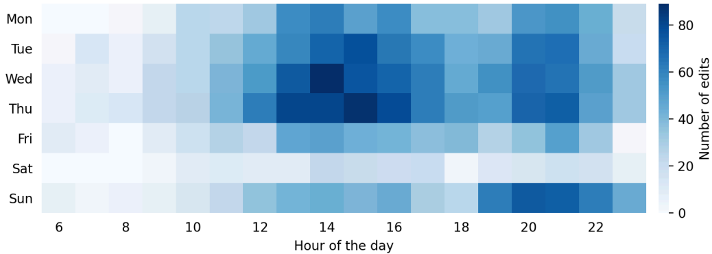
Figure 2: Number of edits by day of the week and hour in the observed sessions
